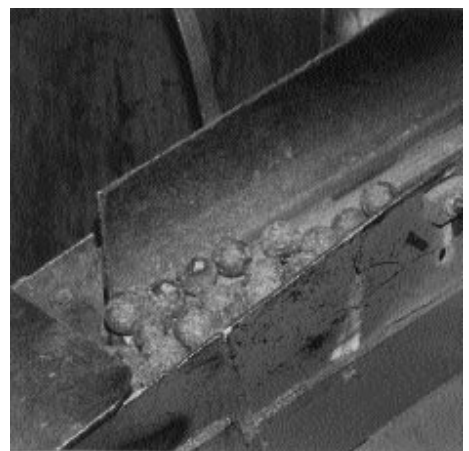
BVS-320 unjamming grinding balls on chute
