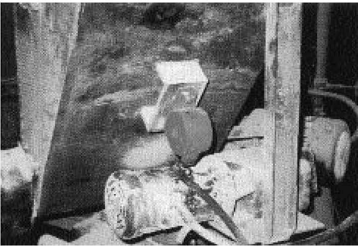
SILENT Turbine mounted to a fly ash chute to keep ash flowing.
